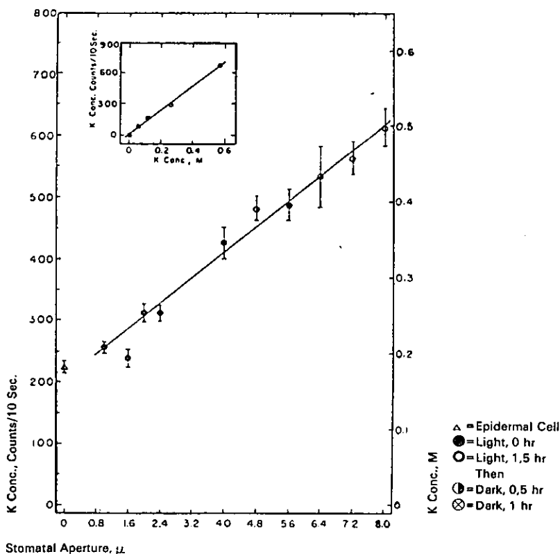
Fig. 2. Relation of potassium concentration in guard cells and stomatal aperture in intact tobacco leaf tissue. Each point shows the mean of 6 to 8 determinations, and the standard deviation of the mean is indicated. The potassium concentration in a typical epidermal cell is also shown. The insert illustrates the relation between counts per 10 sec and potassium concentration of a KCl-impregnated membrane filter that was used to calculate the potassium content of the leaf cells.
